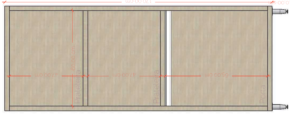
Vista Frontal
